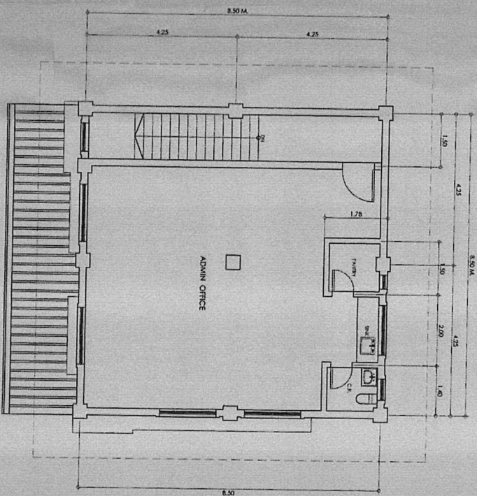
SECOND FLOOR PLAN SCALE 1:50 MTS.
